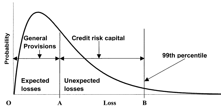
Fig. 1. Probability density functions of loan losses, provisions, and economic capital.
